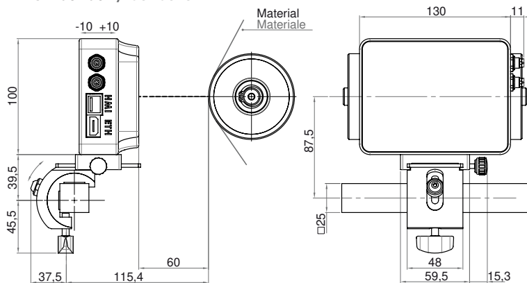
PTS 25 sensor / sensore
